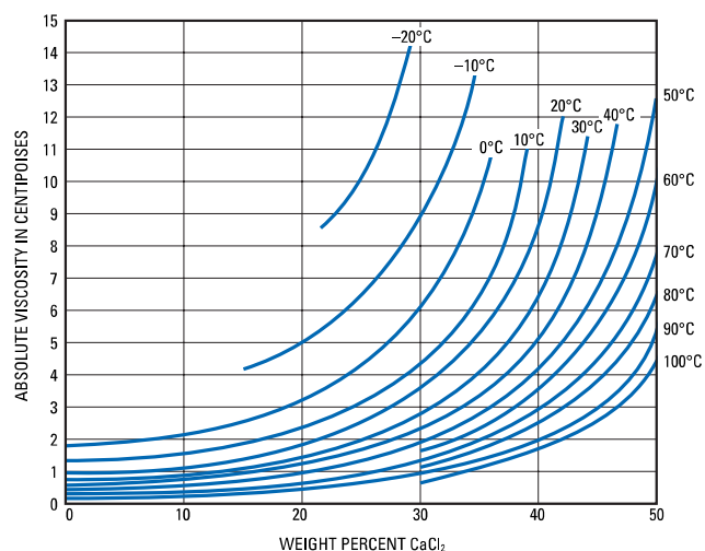
Figure 5: Viscosity of Pure CaCl 2 Solutions
