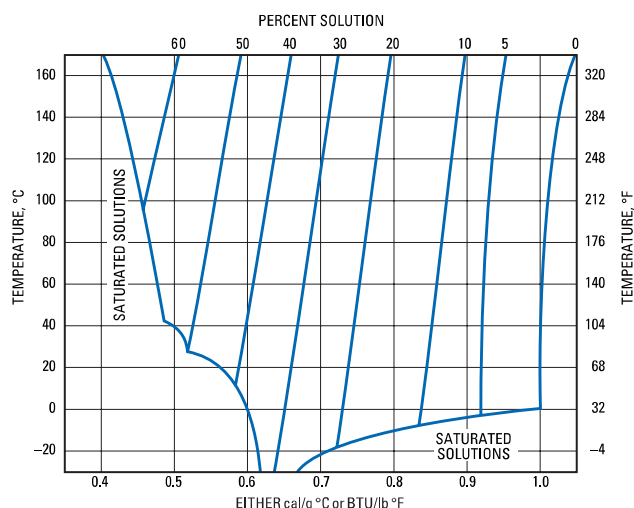
Figure 4: Specific Heat of Aqueous CaCl 2 Solutions
